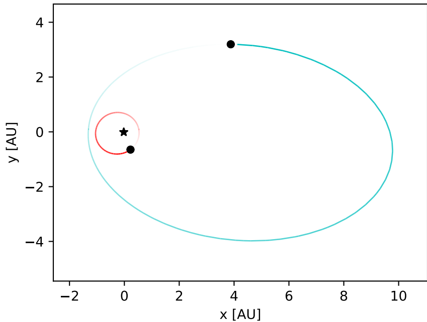
Three-Body System after 100 Years
